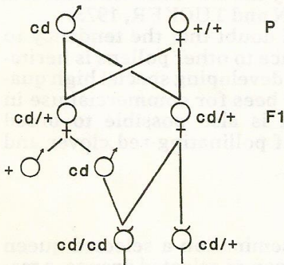
Fig. 32 — Crossing diagram to obtain a mutation. cd =cordovan, t =wild type, F=first generation, p=parental generation
