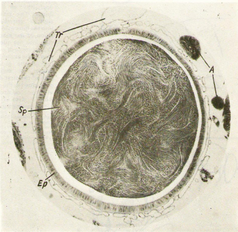
Fig. 9 — Transversal section through the spermatheca of a mated queen A — gland; Ep — spermatheca wall made up of high cells; Sp — spermatozoa gathered in interdependent clusters; Tr — extern cover of tracheae
